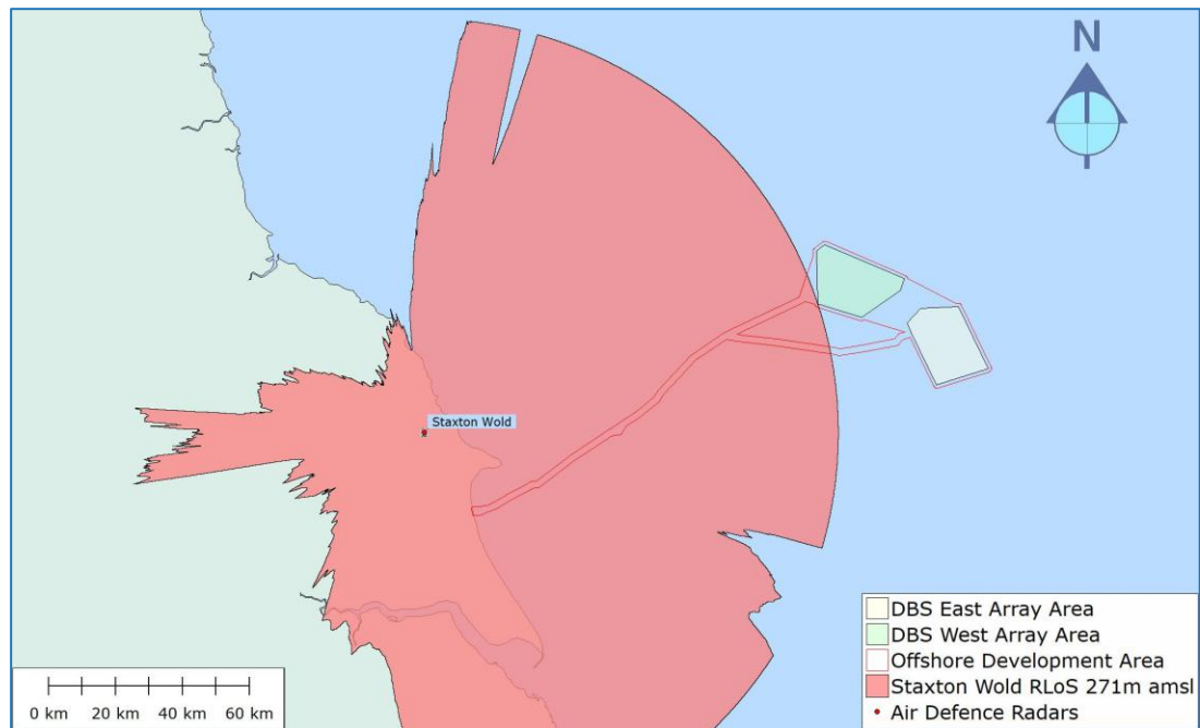
Figure 17: Staxton Wold RLoS 271m amsl
