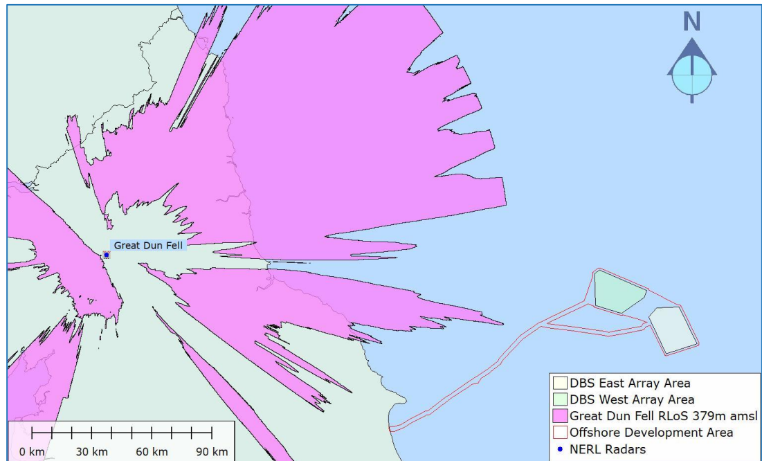
Figure 14: Great Dun Fell RLoS 39679m amsl
