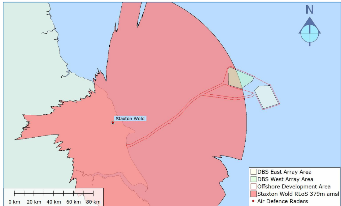
Figure 15: Staxton Wold RLoS 39679m amsl
