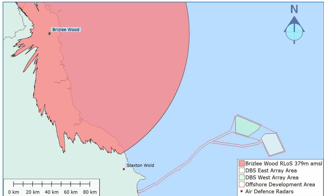
Figure 20: Brizlee Wood RLoS 39679m amsl
