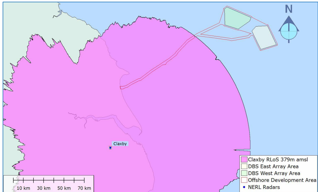
Figure 12: Claxby RLoS 39679m amsl
